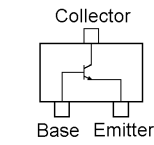
2SC4617 (BR) (Q1040, 1041, 1042) 2SC4915 (QY) (Q1017, 1020, 1021, 1022, 1023, 1028, 1035)
